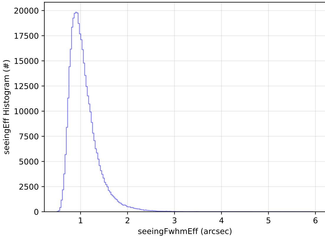
ddf_acor_sf10_lsf20_lsr20_v3.4_10yrs All sky y band: seeingEff Histogram
