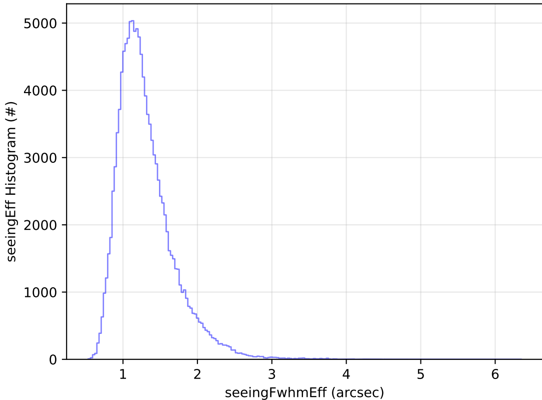
ddf_acor_sf10_ls20_lsr20_v3.4_10yrs All sky u band: seeingEff Histogram
