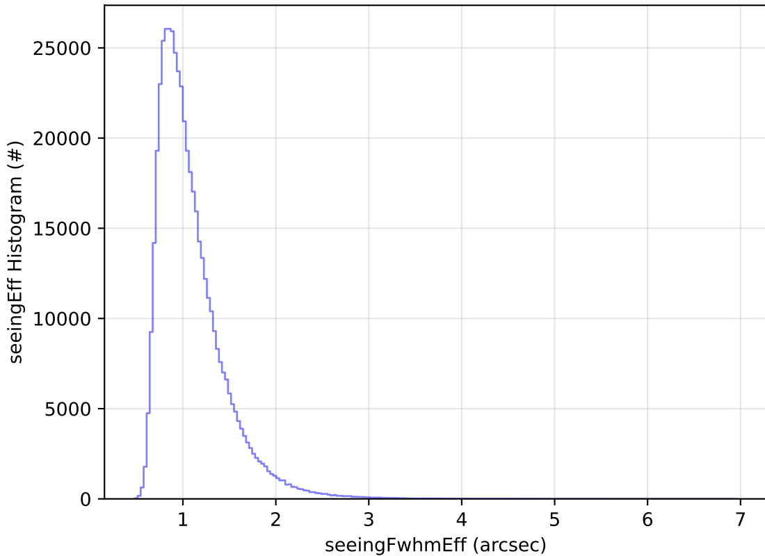
ddf_acor_sf10_lsf20_lsr20_v3.4_10yrs All sky i band: seeingEff Histogram
