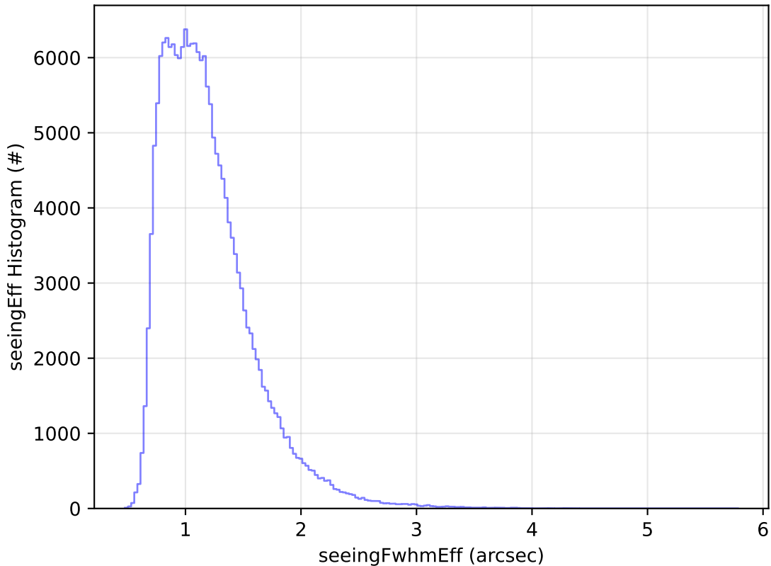
ddf_acor_sf10_ls20_lsr20_v3.4_10yrs All sky g band: seeingEff Histogram
