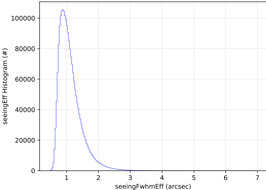
ddf_acor_sf10_lsf20_lsr20_v3.4_10yrs All sky all bands: seeingEff Histogram
