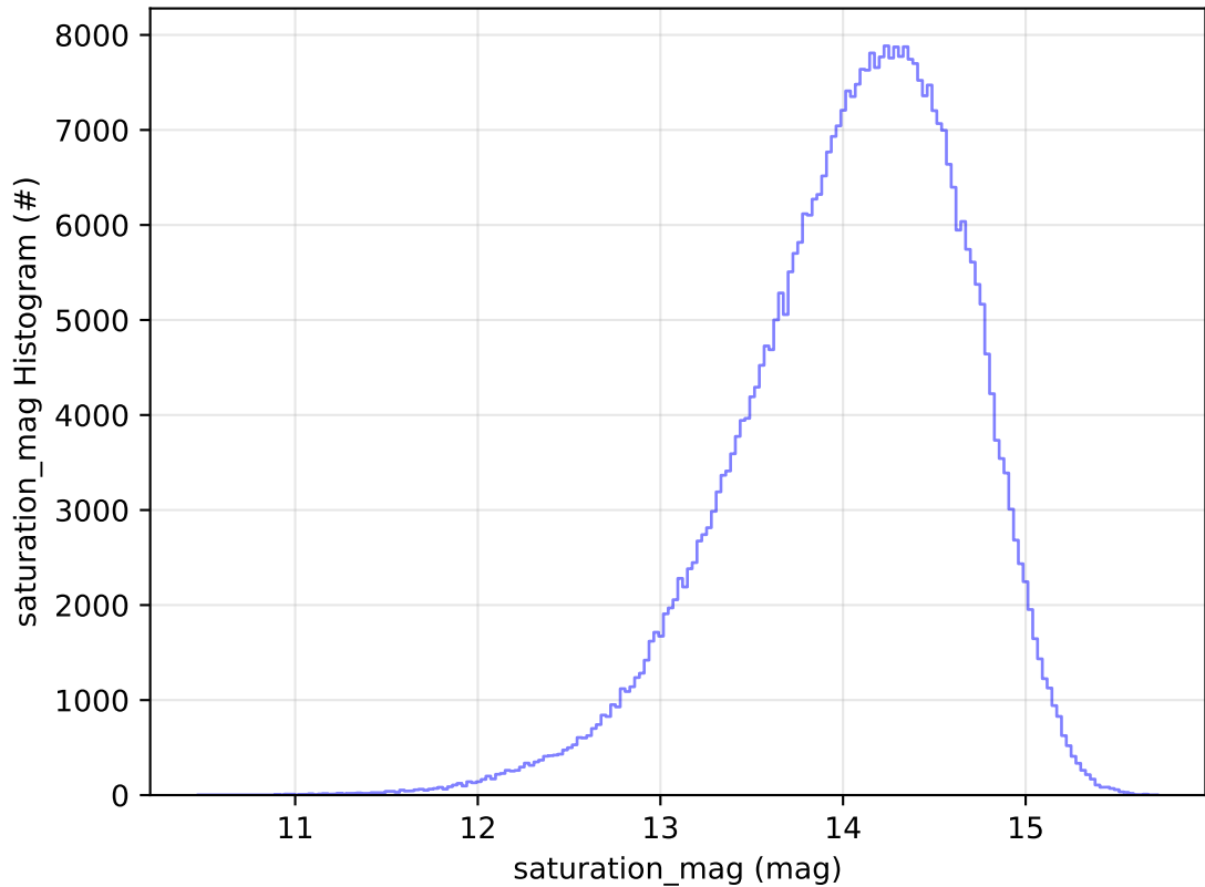
ddf_acor_sf10_lsf20_lsr20_v3.4_10yrs WFD z band: saturation_mag Histogram
