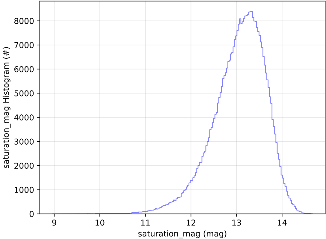
ddf_acor_sf10_lsf20_lsr20_v3.4_10yrs WFD y band: saturation_mag Histogram
