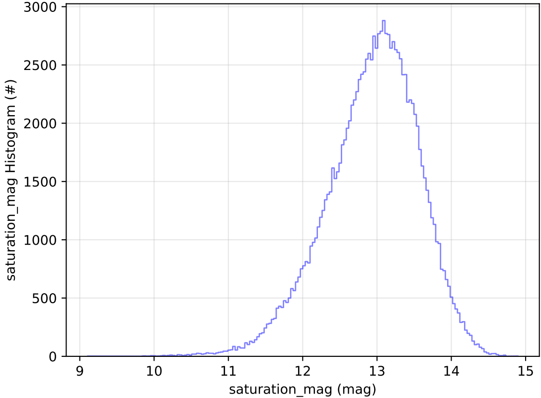
ddf_acor_sf10_lsf20_lsr20_v3.4_10yrs WFD u band: saturation_mag Histogram
