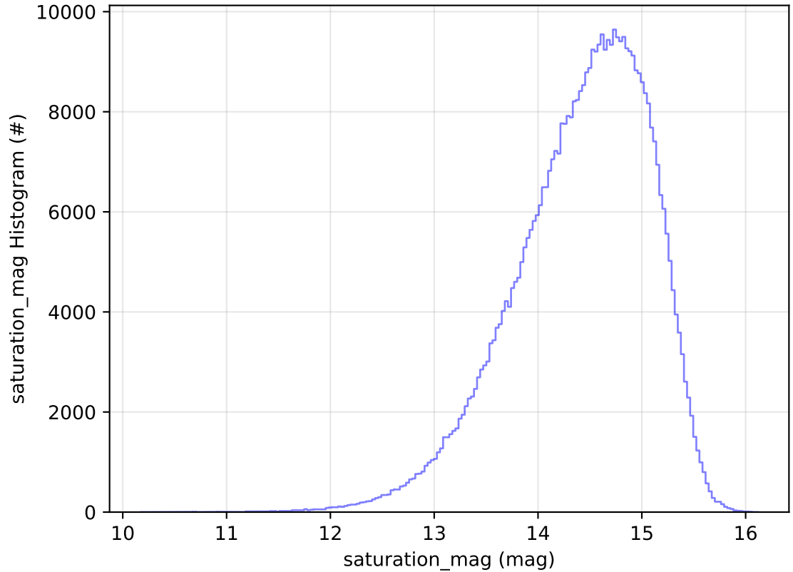
ddf_acor_sf10_lsf20_lsr20_v3.4_10yrs WFD i band: saturation_mag Histogram
