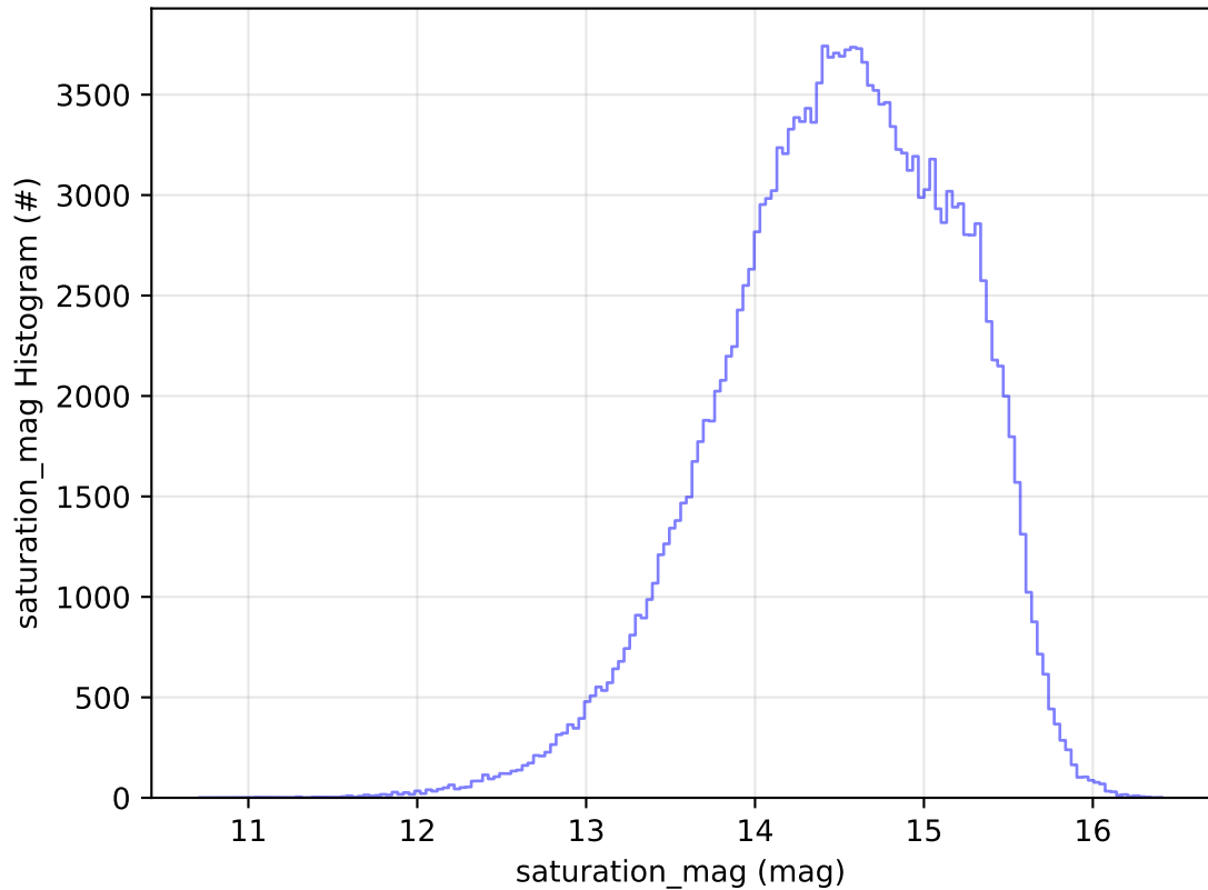
ddf_acor_sf10_lsf20_lsr20_v3.4_10yrs WFD g band: saturation_mag Histogram
