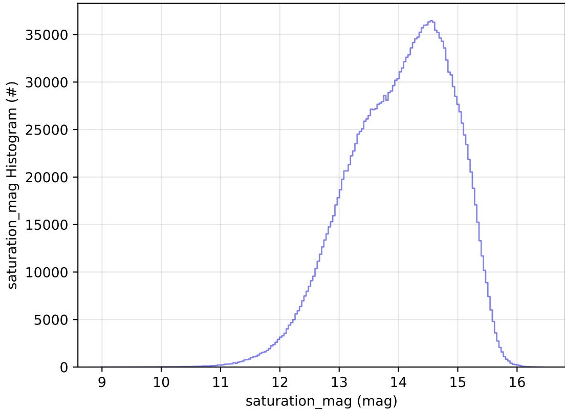
ddf_acor_sf10_lsf20_lsr20_v3.4_10yrs WFD all bands: saturation_mag Histogram
