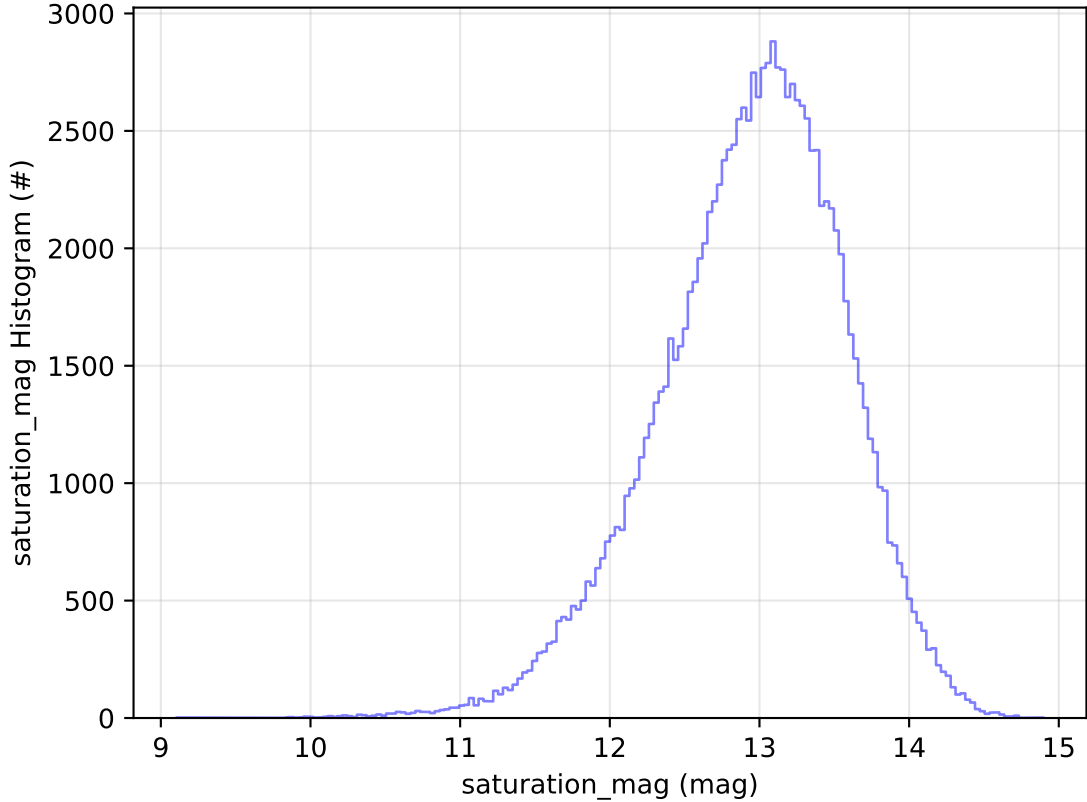
ddf_acor_sf10_lsf20_lsr20_v3.4_10yrs All sky u band: saturation_mag Histogram
