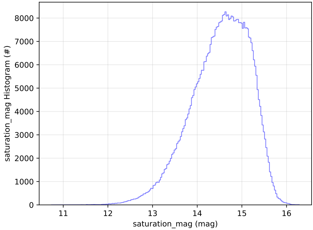
ddf_acor_sf10_lsf20_lsr20_v3.4_10yrs All sky r band: saturation_mag Histogram
