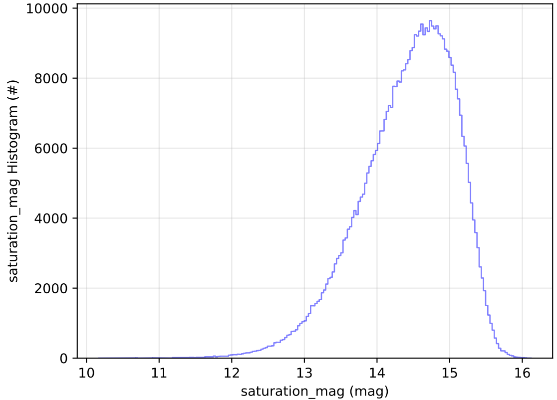
ddf_acor_sf10_lsf20_lsr20_v3.4_10yrs All sky i band: saturation_mag Histogram
