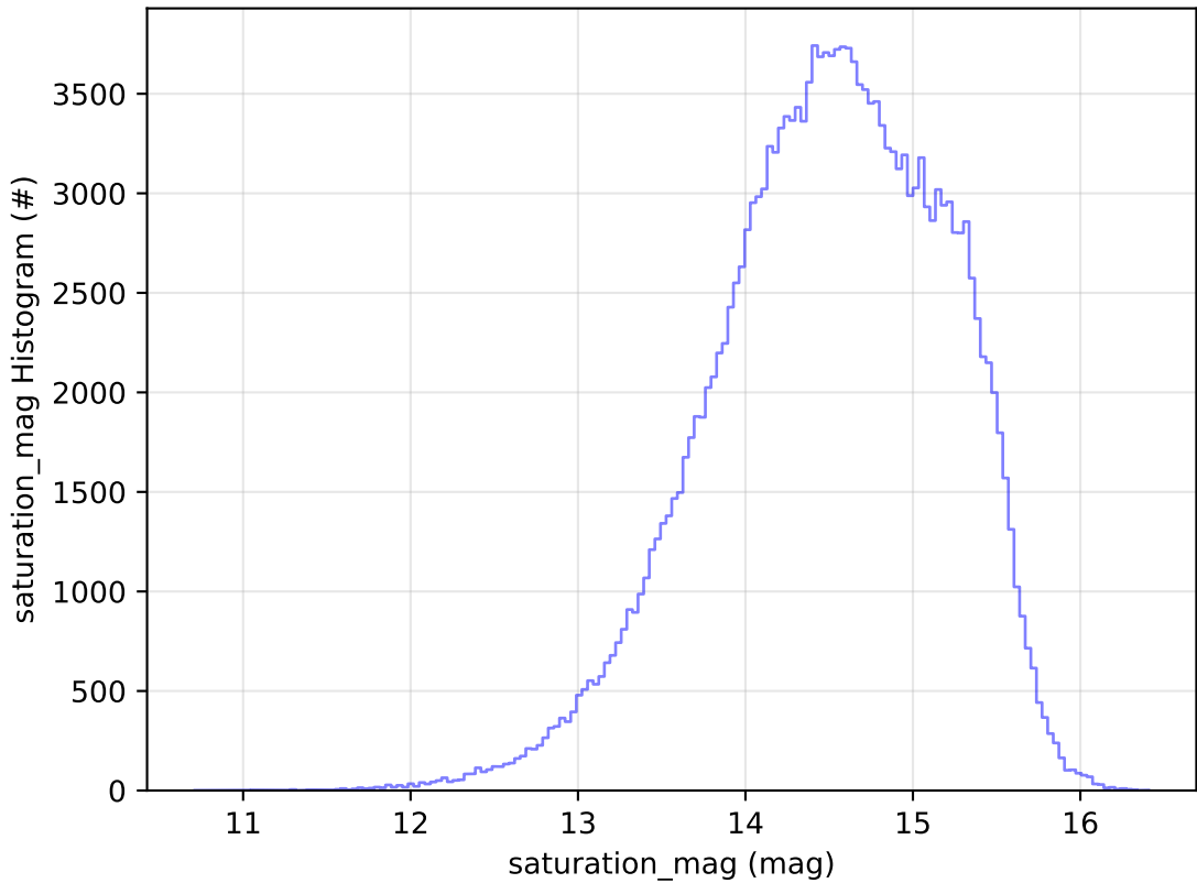
ddf_acor_sf10_lsf20_lsr20_v3.4_10yrs All sky g band: saturation_mag Histogram
