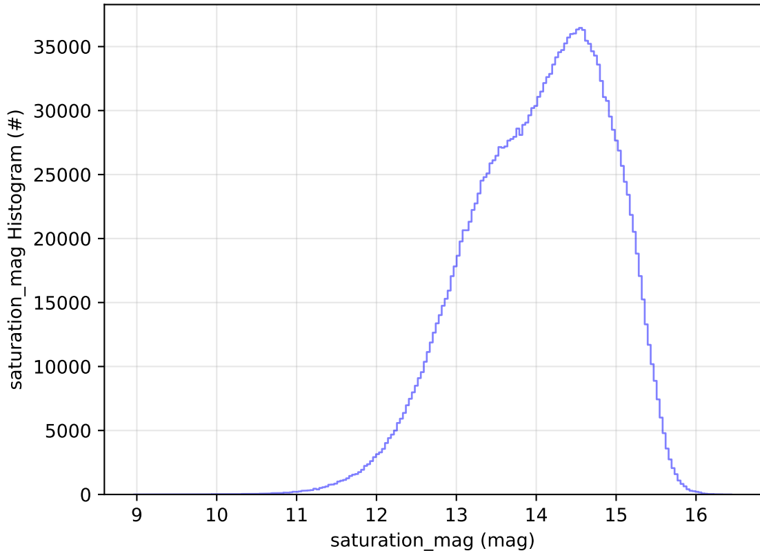
ddf_acor_sf10_lsf20_lsr20_v3.4_10yrs All sky all bands: saturation_mag Histogram
