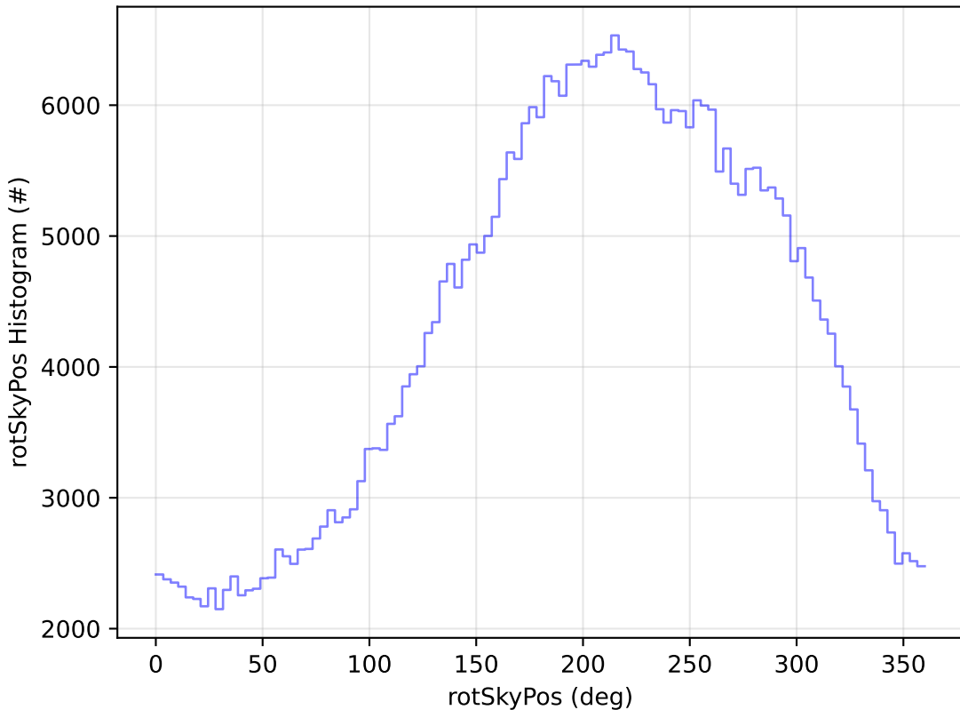
ddf_acor_sf10_lsf20_lsr20_v3.4_10yrs WFD z band: rotSkyPos Histogram
