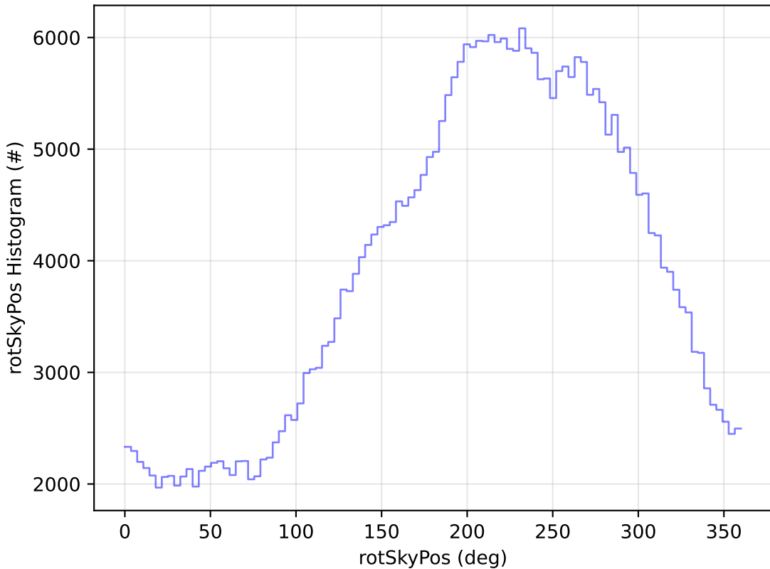
ddf_acor_sf10_lsf20_lsr20_v3.4_10yrs WFD y band: rotSkyPos Histogram
