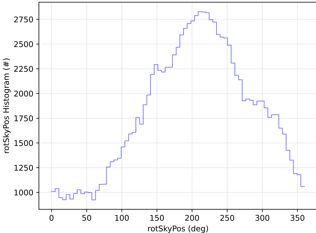
ddf_acor_sf10_lsf20_lsr20_v3.4_10yrs WFD u band: rotSkyPos Histogram
