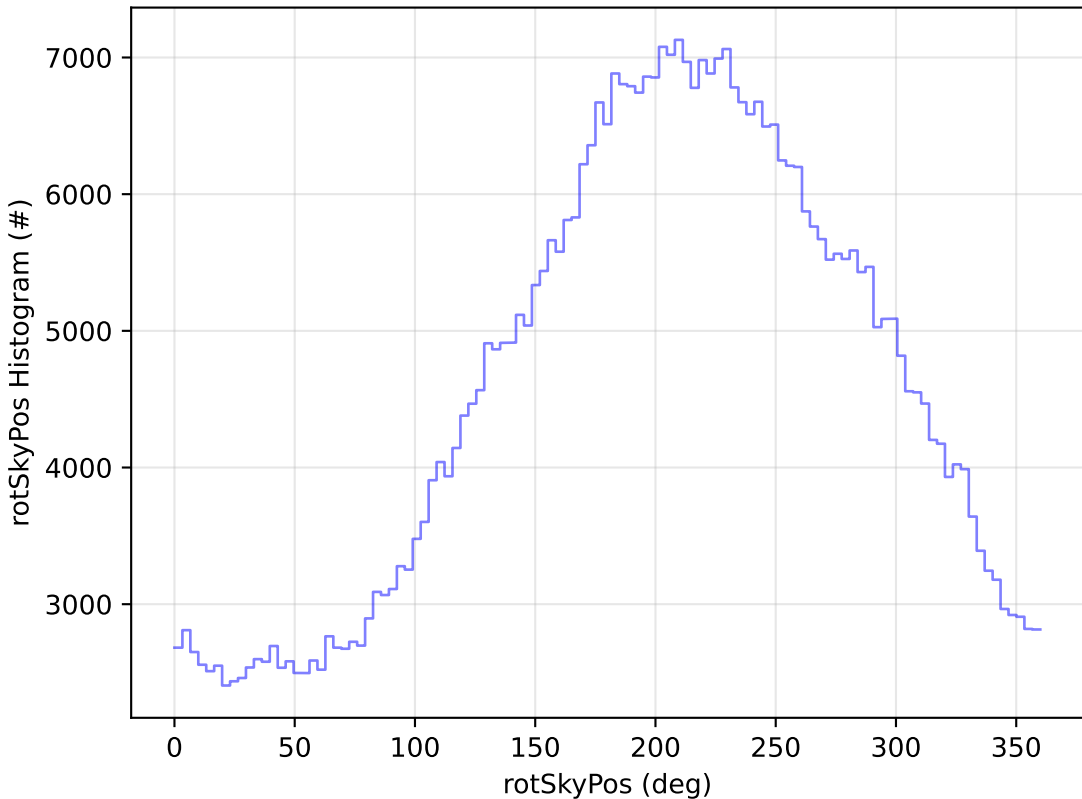
ddf_acor_sf10_lsf20_lsr20_v3.4_10yrs WFD i band: rotSkyPos Histogram
