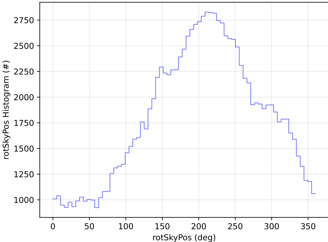
ddf_acor_sf10_lsf20_lsr20_v3.4_10yrs All sky u band: rotSkyPos Histogram
