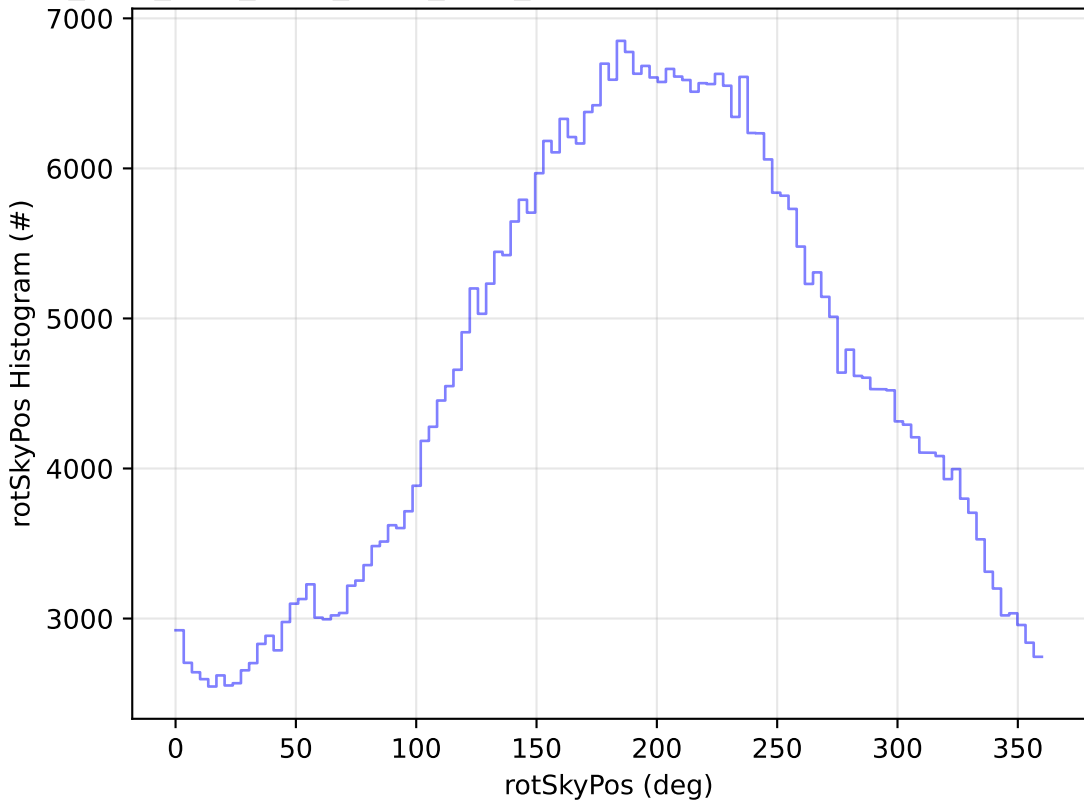
ddf_acor_sf10_ls20_lsr20_v3.4_10yrs All sky r band: rotSkyPos Histogram
