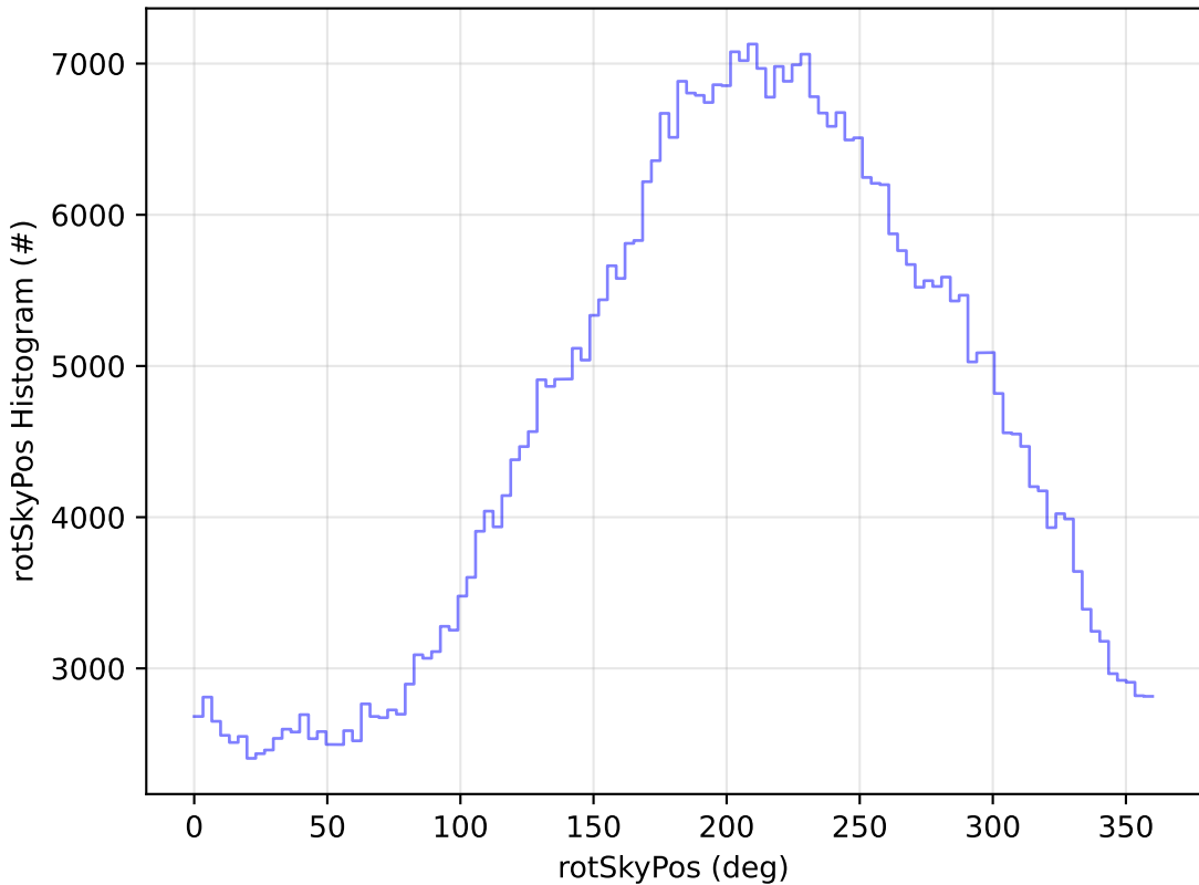
ddf_acor_sf10_lsf20_lsr20_v3.4_10yrs All sky i band: rotSkyPos Histogram
