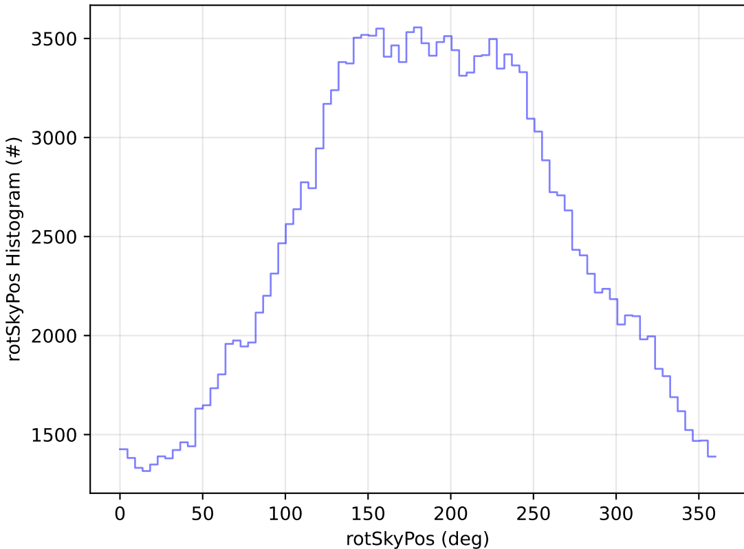
ddf_acor_sf10_lsf20_lsr20_v3.4_10yrs All sky g band: rotSkyPos Histogram
