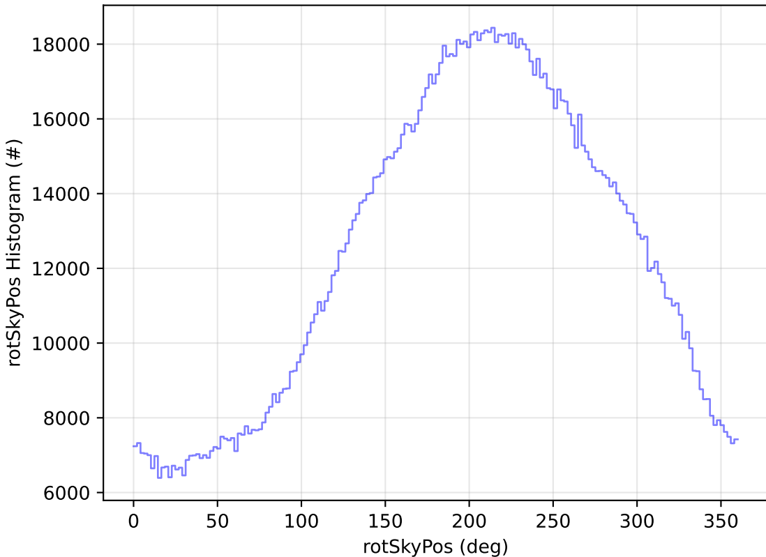
ddf_acor_sf10_lsf20_lsr20_v3.4_10yrs All sky all bands: rotSkyPos Histogram
