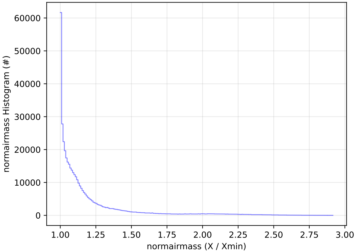
ddf_acor_sf10_lsf20_lsr20_v3.4_10yrs WFD z band: normairmass Histogram
