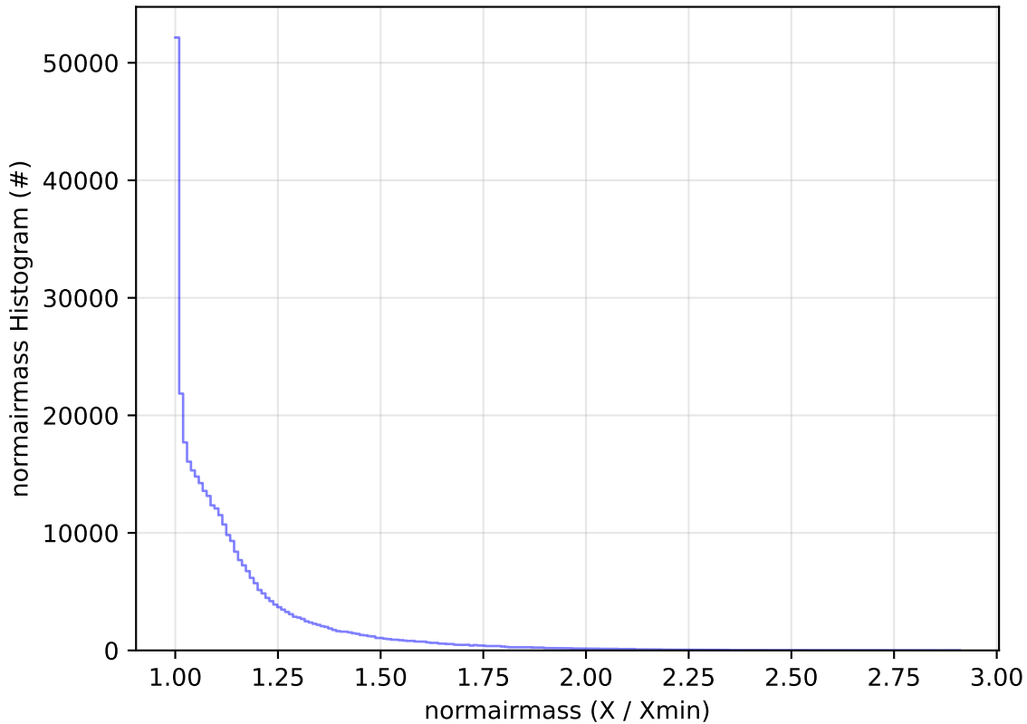
ddf_acor_sf10_lsf20_lsr20_v3.4_10yrs WFD y band: normairmass Histogram
