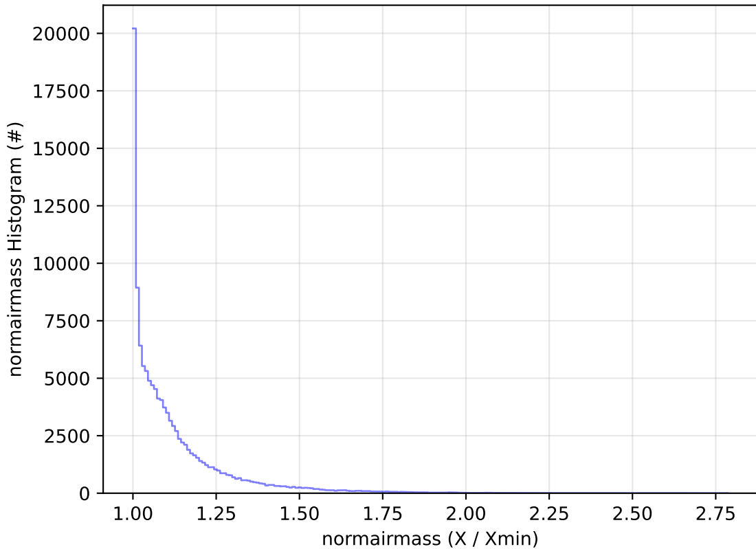
ddf_acor_sf10_lsf20_lsr20_v3.4_10yrs WFD u band: normairmass Histogram
