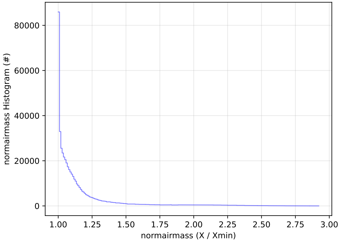
ddf_acor_sf10_lsf20_lsr20_v3.4_10yrs WFD i band: normairmass Histogram
