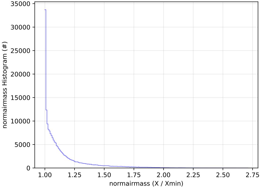
ddf_acor_sf10_lsf20_lsr20_v3.4_10yrs WFD g band: normairmass Histogram
