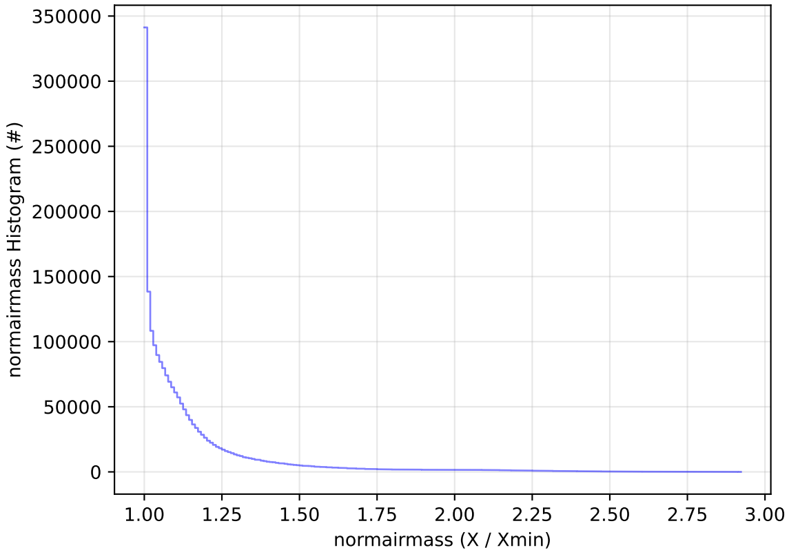
ddf_acor_sf10_lsf20_lsr20_v3.4_10yrs WFD all bands: normairmass Histogram
