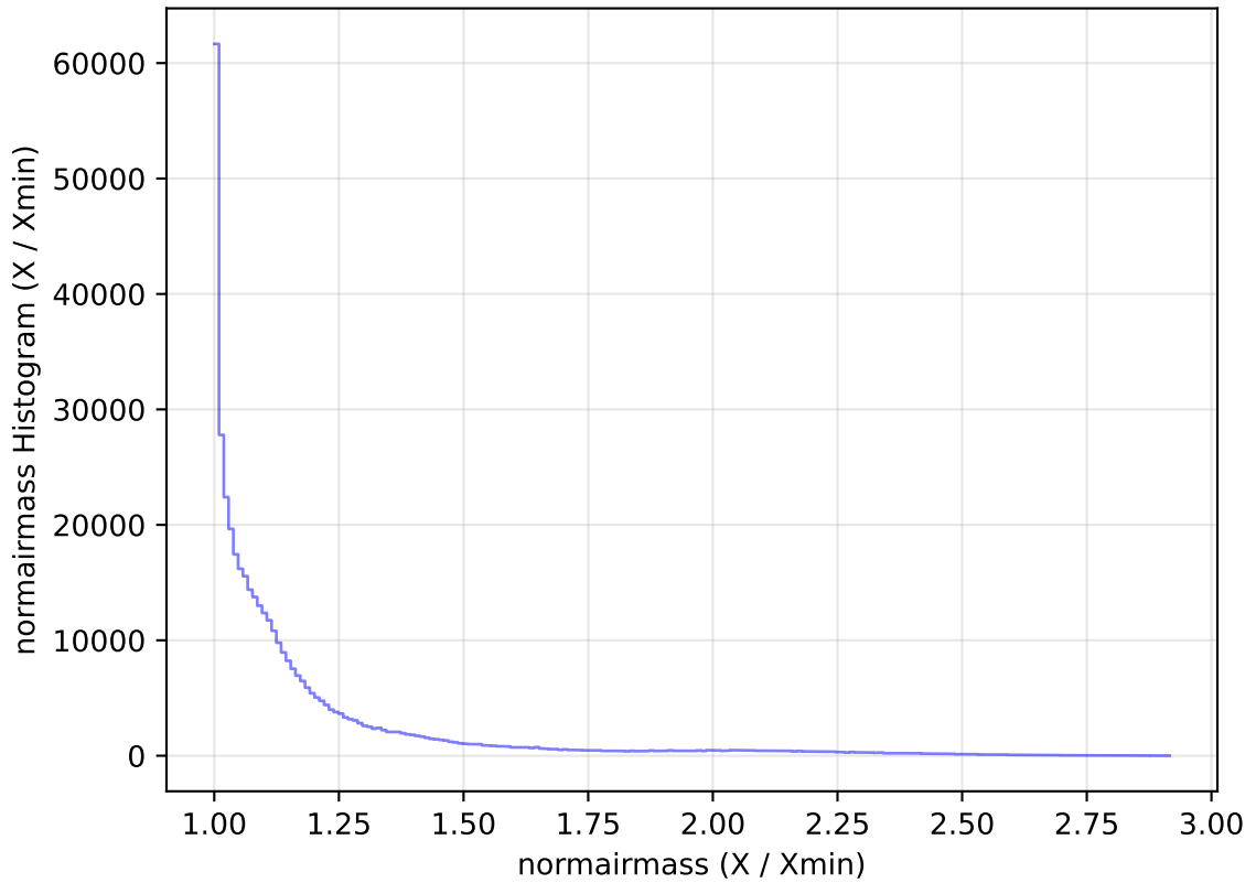
ddf_acor_sf10_lsf20_lsr20_v3.4_10yrs All sky z band: normairmass Histogram
