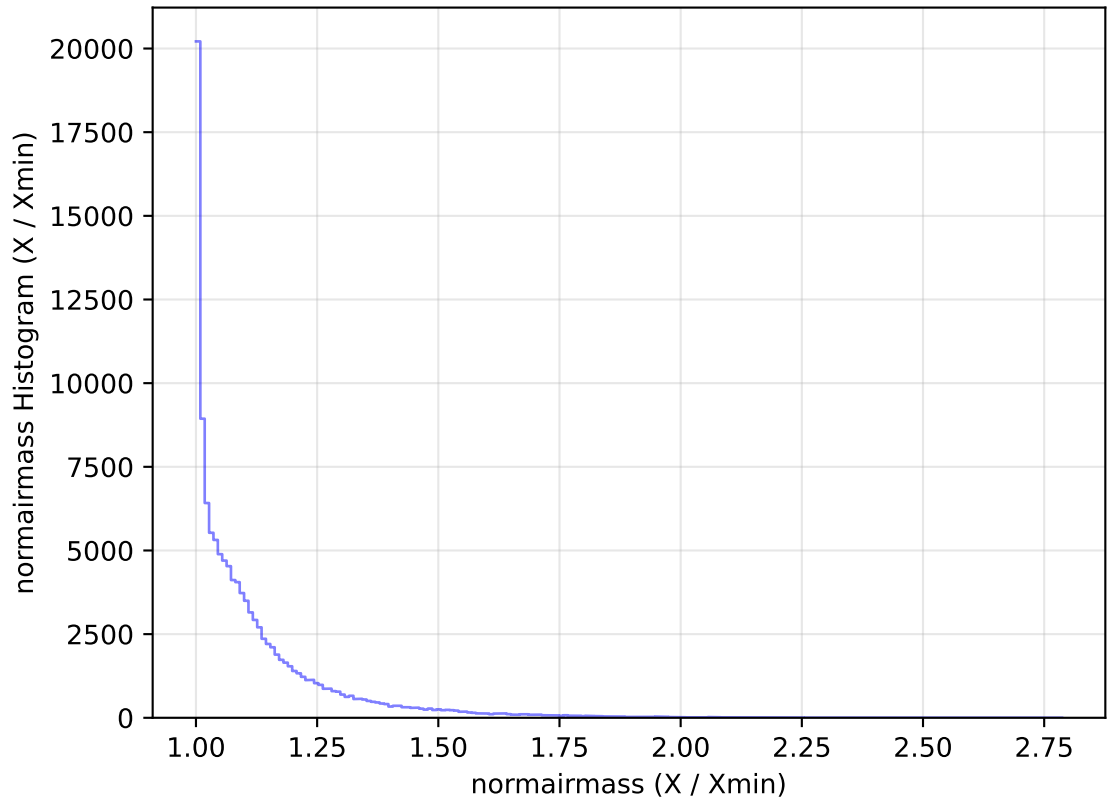
ddf_acor_sf10_lsf20_lsr20_v3.4_10yrs All sky u band: normairmass Histogram
