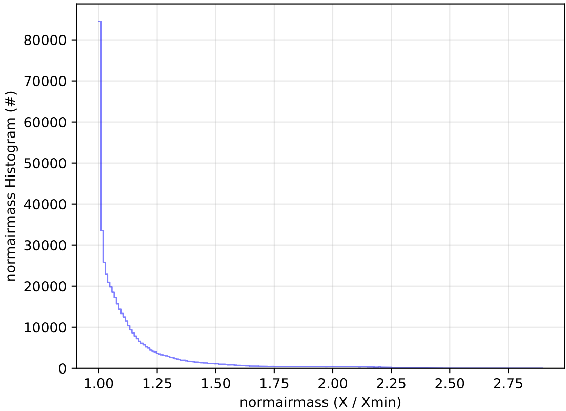
ddf_acor_sf10_lsf20_lsr20_v3.4_10yrs All sky r band: normairmass Histogram
