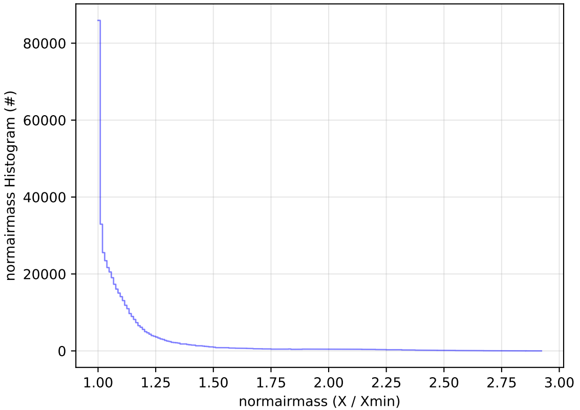
ddf_acor_sf10_lsf20_lsr20_v3.4_10yrs All sky i band: normairmass Histogram
