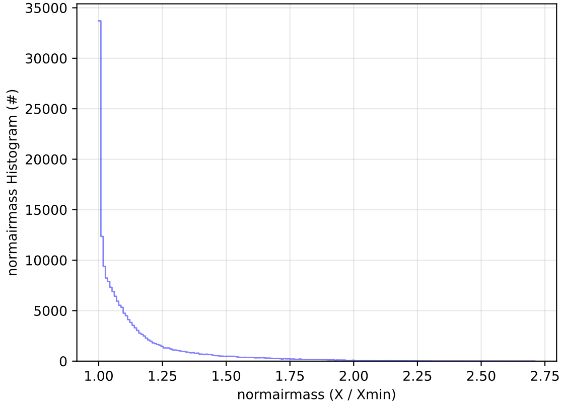
ddf_acor_sf10_lsf20_lsr20_v3.4_10yrs All sky g band: normairmass Histogram
