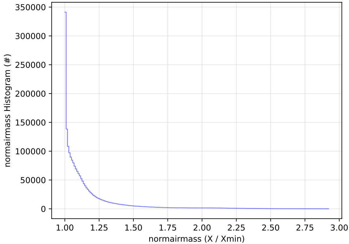
ddf_acor_sf10_lsf20_lsr20_v3.4_10yrs All sky all bands: normairmass Histogram
