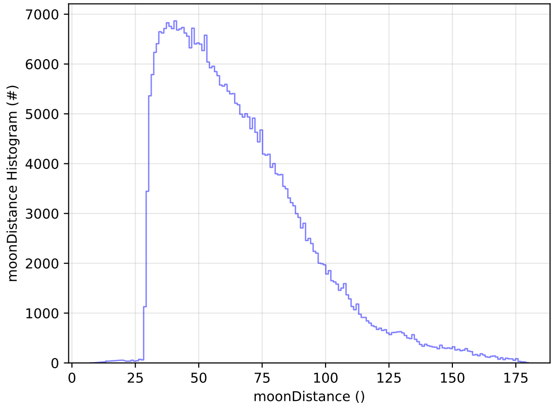
ddf_acor_sf10_lsf20_lsr20_v3.4_10yrs WFD y band: moonDistance Histogram
