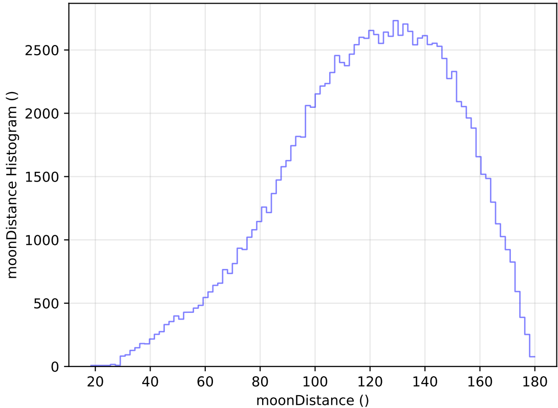
ddf_acor_sf10_lsf20_lsr20_v3.4_10yrs WFD u band: moonDistance Histogram
