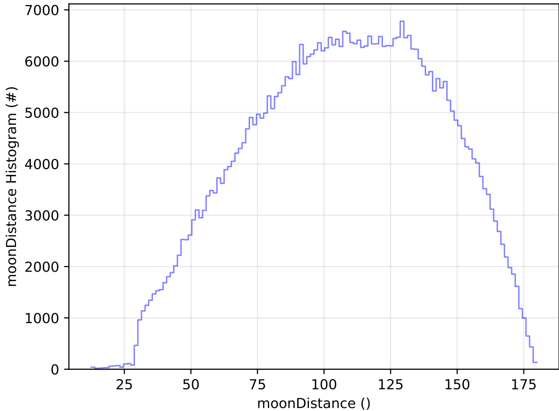
ddf_acor_sf10_lsf20_lsr20_v3.4_10yrs WFD r band: moonDistance Histogram
