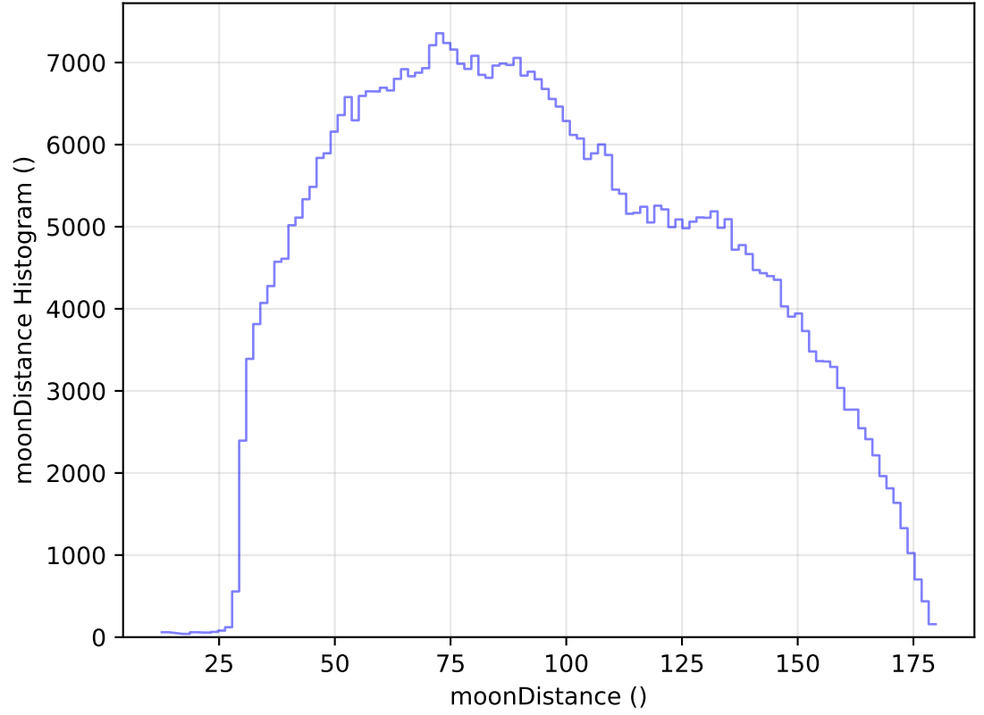
ddf_acor_sf10_lsf20_lsr20_v3.4_10yrs WFD i band: moonDistance Histogram
