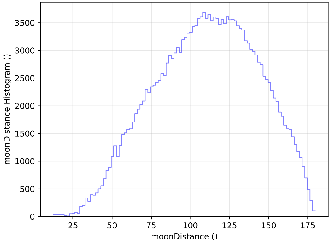
ddf_acor_sf10_lsf20_lsr20_v3.4_10yrs WFD g band: moonDistance Histogram
