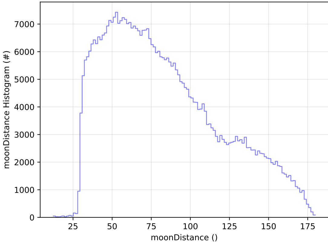
ddf_acor_sf10_lsf20_lsr20_v3.4_10yrs All sky z band: moonDistance Histogram
