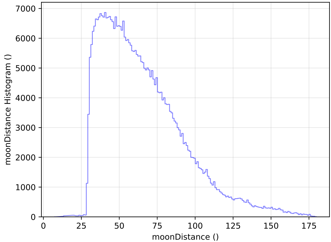
ddf_acor_sf10_lsf20_lsr20_v3.4_10yrs All sky y band: moonDistance Histogram
