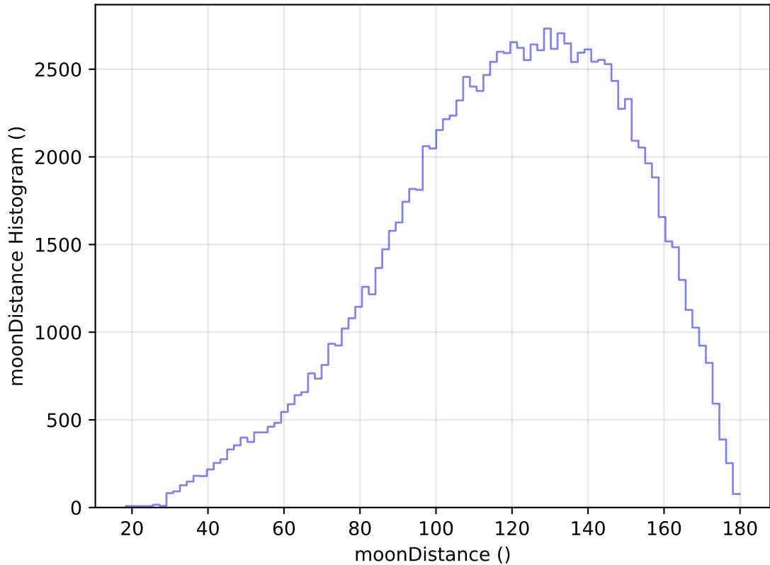
ddf_acor_sf10_lsf20_lsr20_v3.4_10yrs All sky u band: moonDistance Histogram
