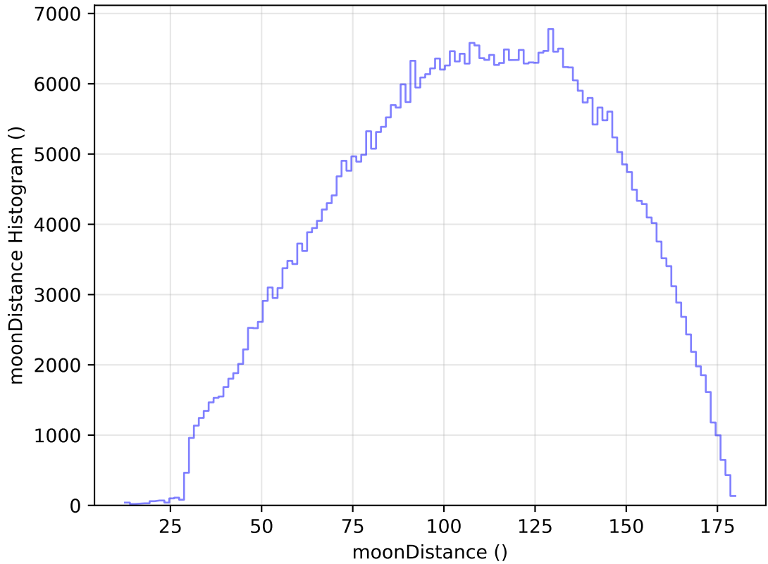
ddf_acor_sf10_lsf20_lsr20_v3.4_10yrs All sky r band: moonDistance Histogram
