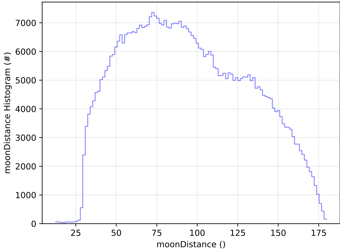
ddf_acor_sf10_lsf20_lsr20_v3.4_10yrs All sky i band: moonDistance Histogram
