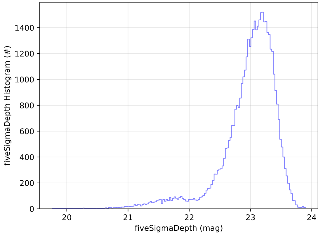
ddf_acor_sf10_lsf20_lsr20_v3.4_10yrs Yr 1 z band: fiveSigmaDepth Histogram
