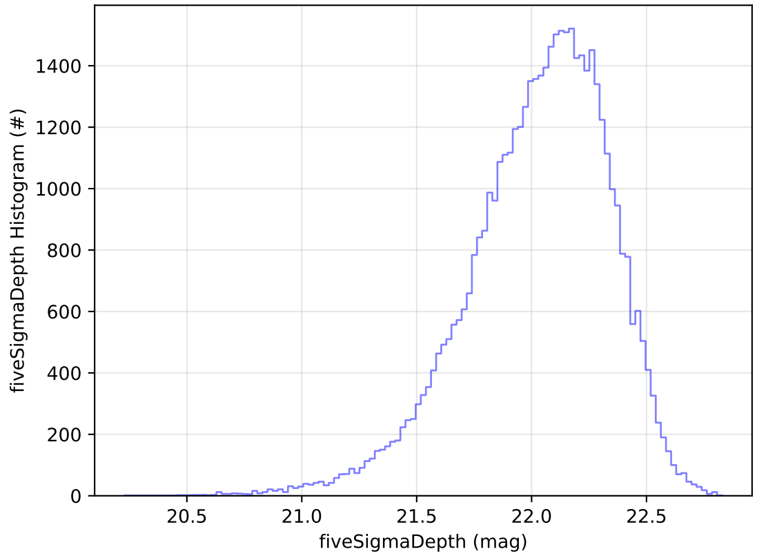
ddf_acor_sf10_lsf20_lsr20_v3.4_10yrs Yr 1 y band: fiveSigmaDepth Histogram
