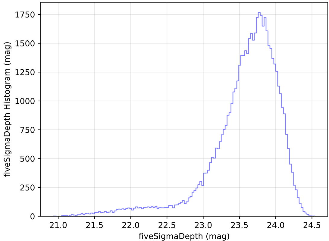
ddf_acor_sf10_lsf20_lsr20_v3.4_10yrs Yr 1 i band: fiveSigmaDepth Histogram
